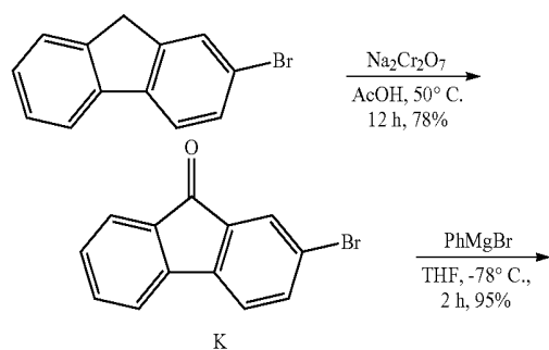
Reaction Scheme 9
